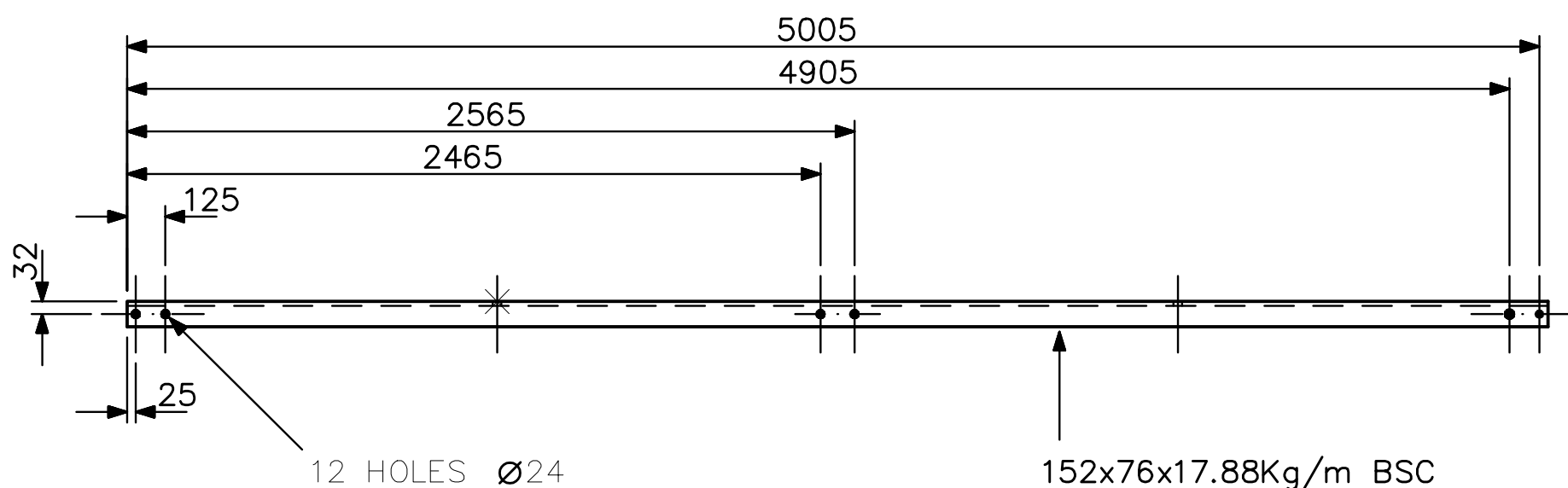
PLAN
